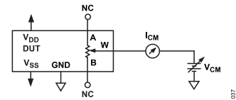
Figure 30. Common-Mode Leakage Current
