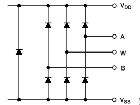
Figure 38. Maximum Terminal Voltages Set by V_{DD} and V_{SS}
