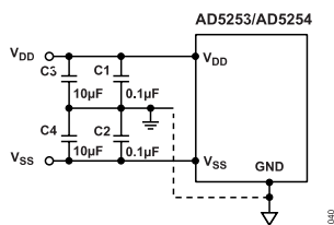
Figure 40. Power Supply-Bypassing Configuration
