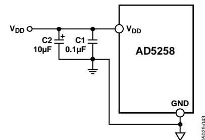
Figure 42. Power Supply Bypassing
