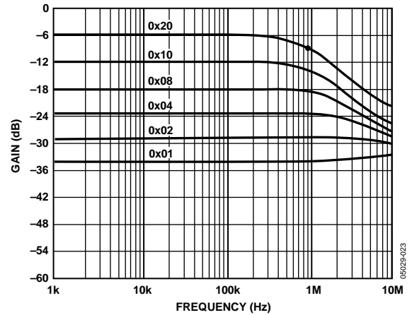
Figure 22. Gain vs. Frequency vs. Code, R AB = 10 kΩ
