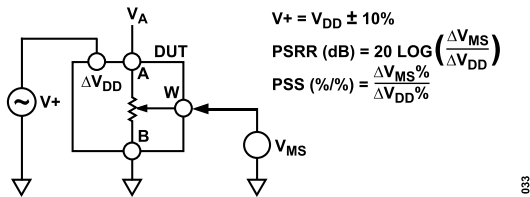
Figure 35. Test Circuit for Power Supply Sensitivity (PSS, PSSR)
