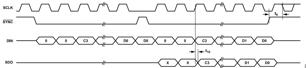
Figure 4. Read Timing Diagram (CPOL = 0, CPHA = 1)
