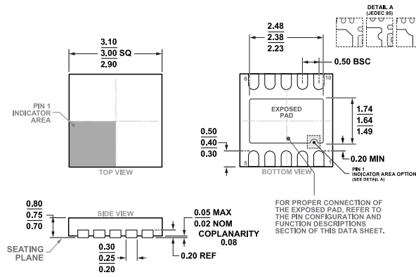
Figure 49. 10-Lead Frame Chip Scale Package [LFCSP] 3 mm x 3 mm Body and 0.75 mm Package Height (CP-10-9) Dimensions shown in millimeters
