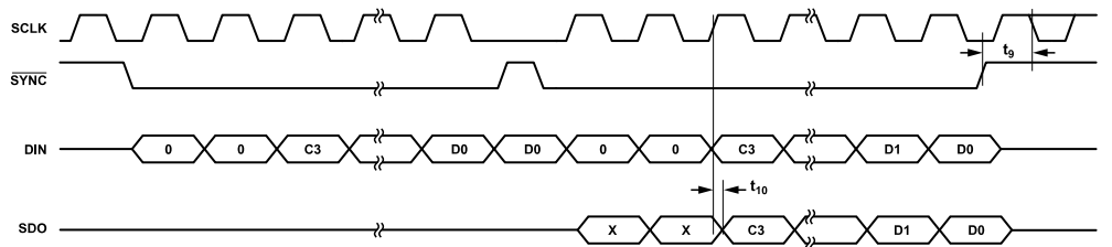
Figure 4. Read Timing Diagram (CPOL = 0, CPHA = 1)
