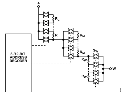
Figure 45. Simplified RDAC Circuit
