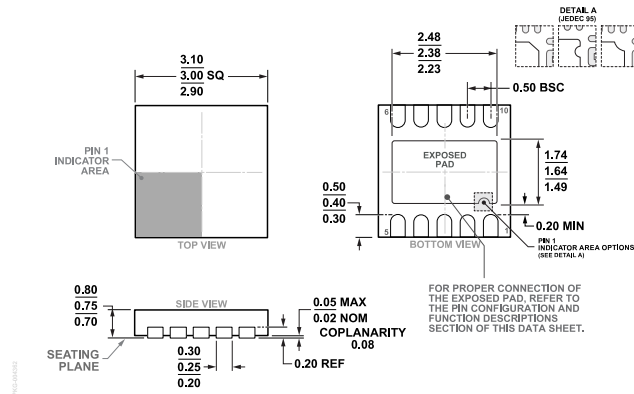
Figure 49. 10-Lead Frame Chip Scale Package [LFCSP] 3 mm x 3 mm Body and 0.75 mm Package Height (CP-10-9) Dimensions shown in millimeters
