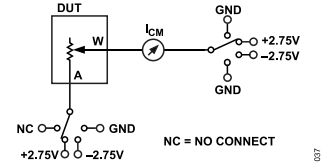
Figure 43. Common Leakage Current
