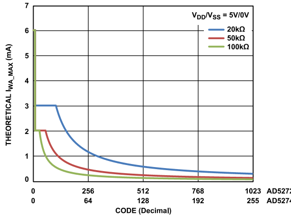
Figure 25. Theoretical Maximum Current vs. Code
