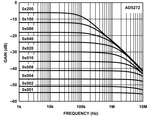
Figure 27. 50 kΩ Gain vs. Code vs. Frequency
