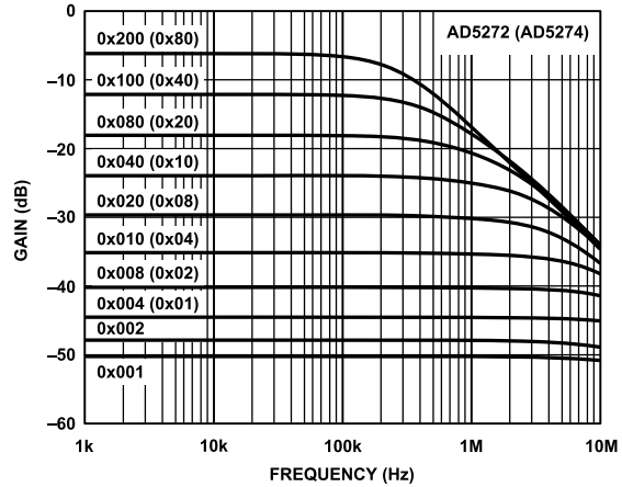
Figure 26. 20 kΩ Gain vs. Code vs. Frequency
