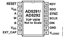
Figure 5. Pin Configuration
