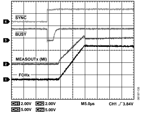
Figure 43. FV Settling, 0 \text{V} to 5 \text{V} , \pm 2 \text{mA} Range, C_{\text{LOAD}} = 220 \text{pF} , CCOMP_x = 100 \text{pF} , R_{\text{LOAD}} = 5.6 \text{k}\Omega
