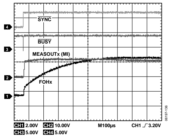
Figure 44. FV Settling, 0 \text{V} to 5 \text{V} , \pm 5 \mu\text{A} Range, C_{\text{LOAD}} = 220 \text{pF} , CCOMP_x = 100 \text{pF} , R_{\text{LOAD}} = 1 \text{M}\Omega
