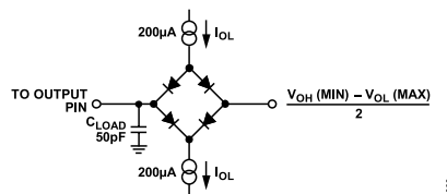
Figure 3. Load Circuit for CMOS
