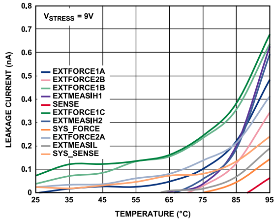
Figure 21. Leakage Current vs. Temperature, V STRESS = 9 V
