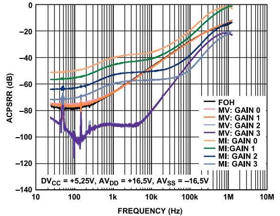
Figure 49. ACPSRR of AVSS vs. Frequency
