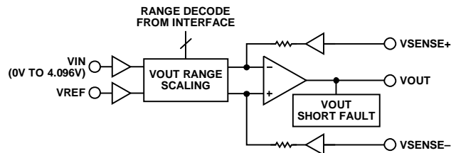
Figure 54. Voltage Output
