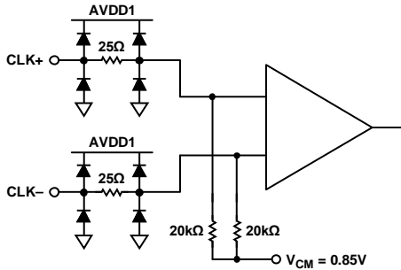
Figure 64. Clock Inputs
