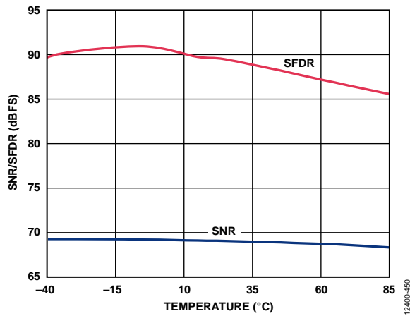
Figure 61. SNR/SFDR vs. Temperature, f_{IN} = 170.3 MHz
