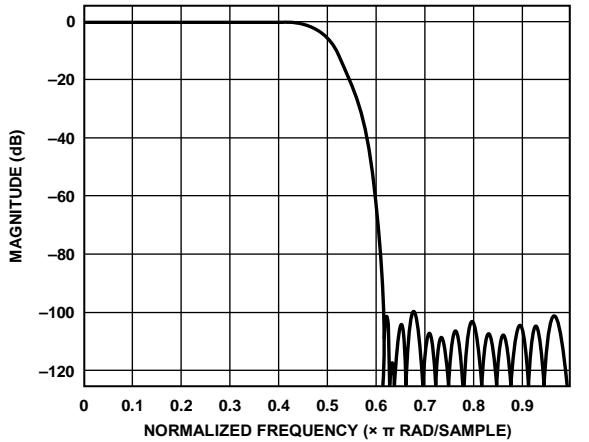
Figure 70. HB1 Filter Response
