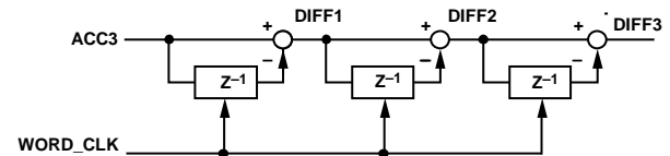
Figure 26. Differentiator
