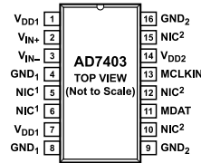
Figure 5. AD7403 Pin Configuration
