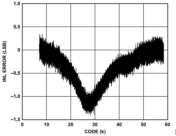
Figure 14. AD7403-8 Typical INL Error
