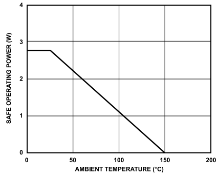
Figure 3. AD7403 Thermal Derating Curve, Dependence of Safety Limiting Values with Case Temperature per DIN V VDE V 0884-10
