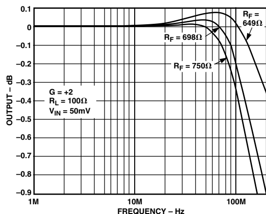
TPC 8. 0.1 dB Flatness, R Package (for N Package Add 50 Ω to R_F )
