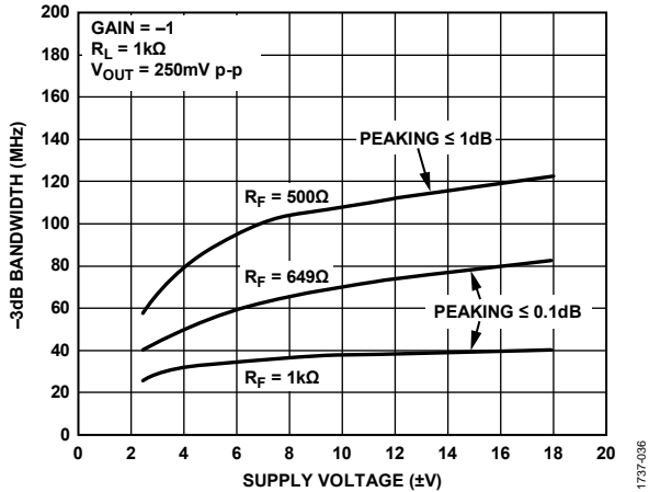
Figure 38. -3 dB Bandwidth vs. Supply Voltage, Gain = -1, R_L = 1 k\Omega
