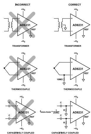
Figure 51. Creating an I_{BIAS} Path
