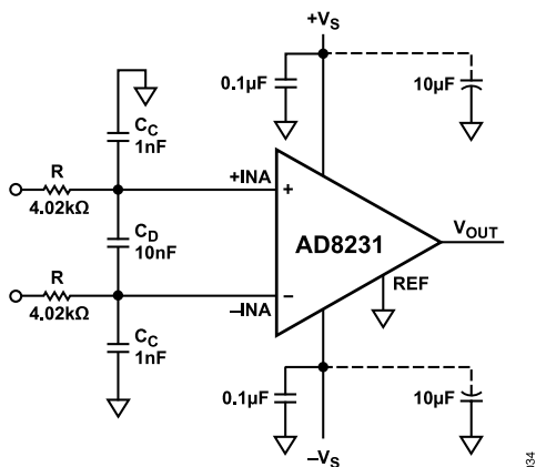
Figure 52. RFI Suppression
