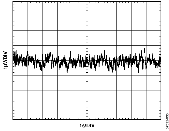
Figure 37. 0.1 Hz to 10 Hz Voltage Noise
