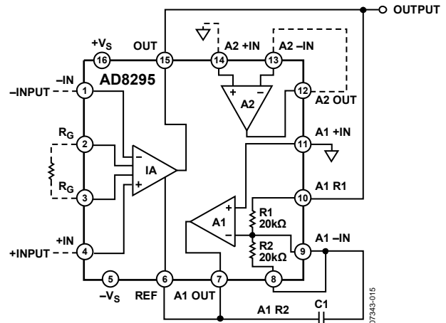
Figure 70. AC-Coupled Connection
