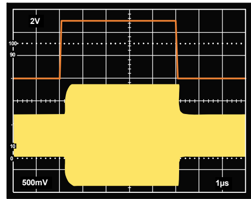
Figure 48 High/Low Response Time
