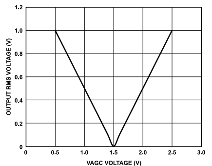
Figure 45. Output RMS Voltage vs. VAGC
