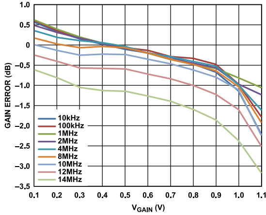
Figure 10. Gain Error vs. V_{GAIN} over Frequency
