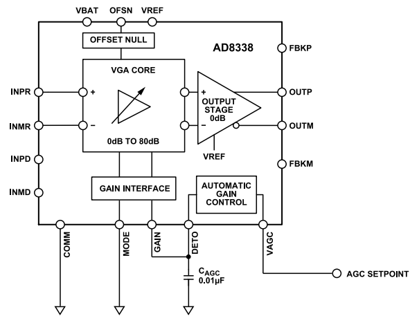
Figure 46. AD8338 Configured as an AGC Amplifier
