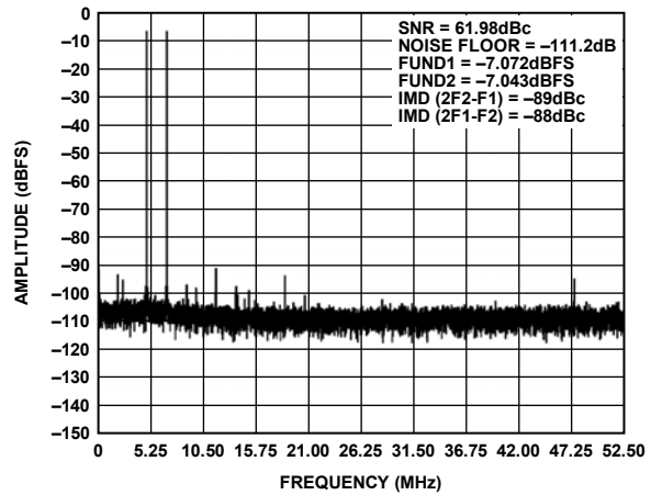
Figure 37. Two Tone Distortion AD8352 Driving AD9445, Encode Clock at 105 MHz with f_c at 100 MHz ( A_v = 10 dB), Analog In = 98 MHz and 101 MHz, See Figure 34
