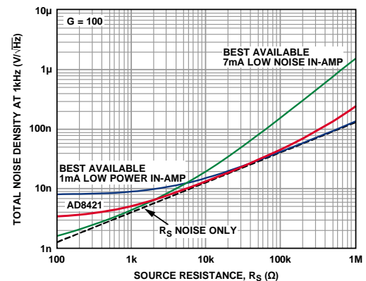
Figure 2. Noise Density vs. Source Resistance
