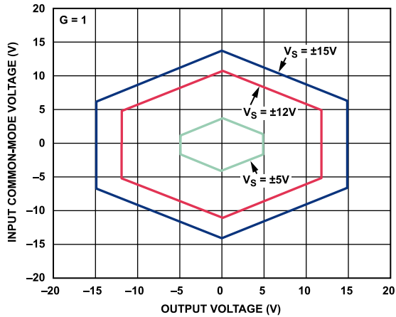
Figure 11. Input Common-Mode Voltage vs. Output Voltage (G = 1), V_S = \pm 15\text{ V} , V_S = \pm 12\text{ V} , V_S = \pm 5\text{ V}
