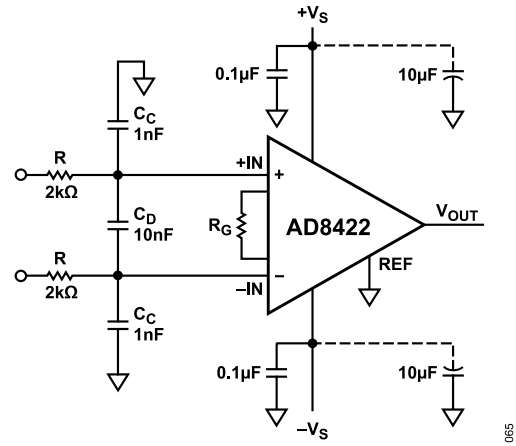
Figure 63. RFI Suppression
