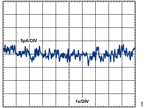
Figure 44. 0.1 Hz to 10 Hz Current Noise
