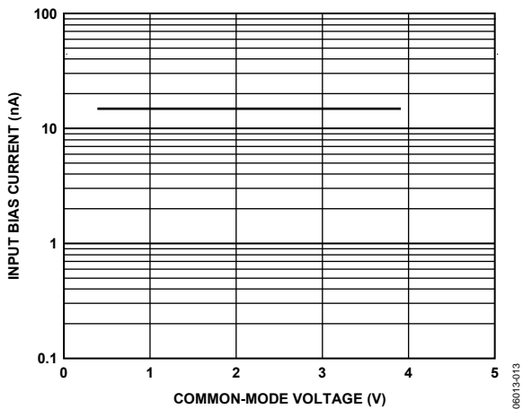
Figure 12. Input Bias Current at V_{POS} , V_{NEG} vs. Common-Mode Voltage, T_A = 25^\circ C
