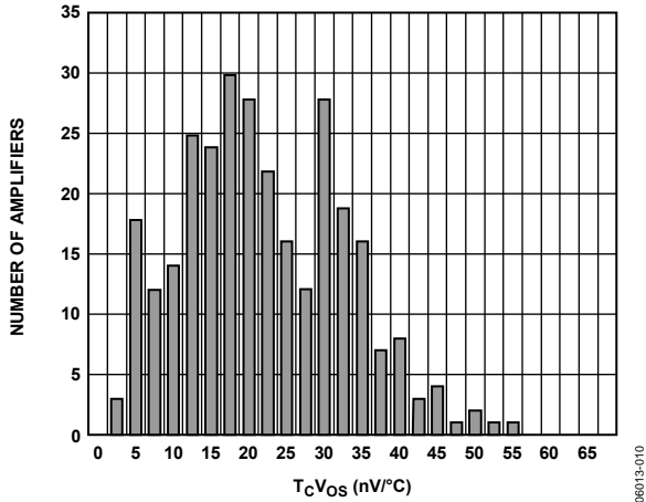
Figure 10. T_C V_{OS} at V_{SY} = 2.7 V , -40^\circ C \leq T_A \leq +125^\circ C
