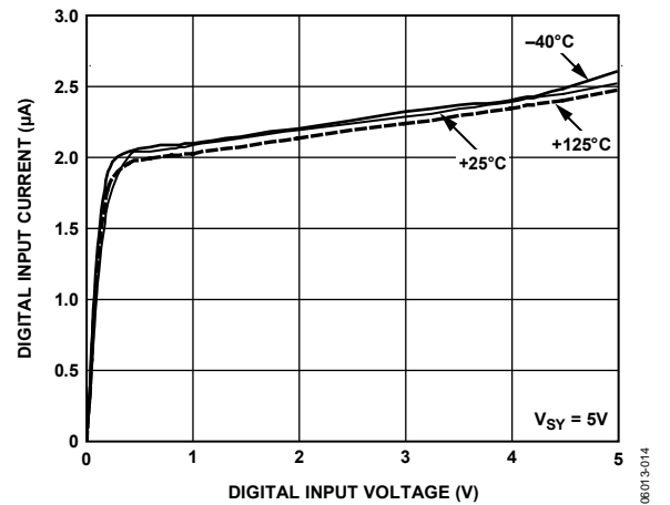
Figure 14. Digital Input Current vs. Digital Input Voltage (Pin 4)
