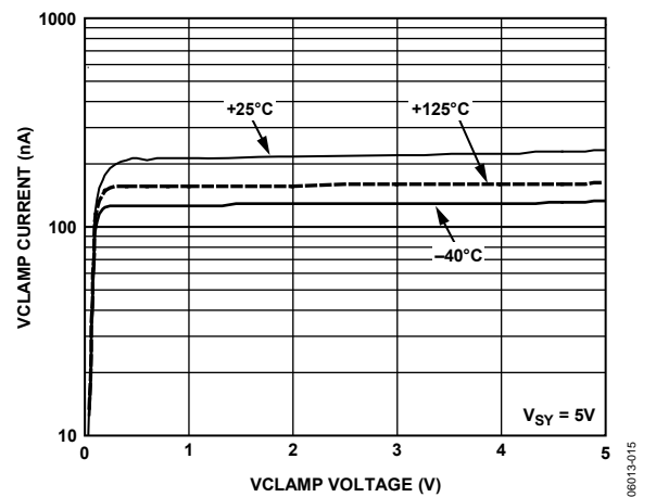
Figure 15. V_{CLAMP} Current over Temperature at V_{SY} = 5\text{ V} vs. V_{CLAMP} Voltage
