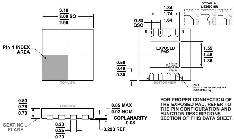
COMPLIANT TO JEDEC STANDARDS MO-229-WEED-4 Figure 61. 8-Lead Lead Frame Chip Scale Package [LFCSP] 3 mm x 3 mm Body and 0.75 mm Package Height (CP-8-13) Dimensions shown in millimeters
