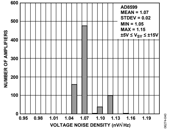
Figure 43. Voltage Noise Density at 1 kHz
