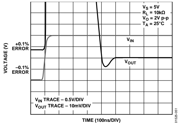
Figure 51. Settling Time
