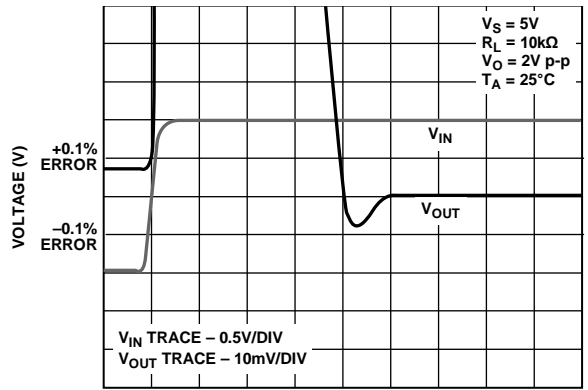
Figure 51. Settling Time
