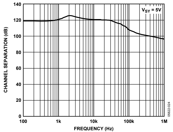
Figure 26. Channel Separation
