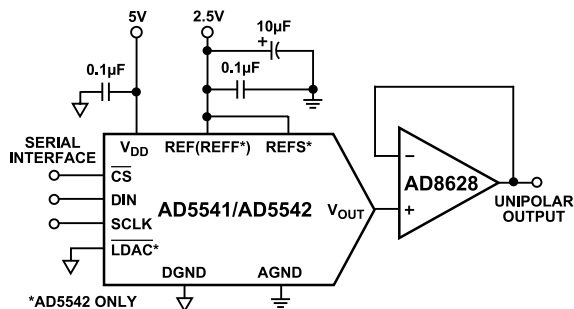
Figure 64. AD8628 Used as an Output Amplifier
