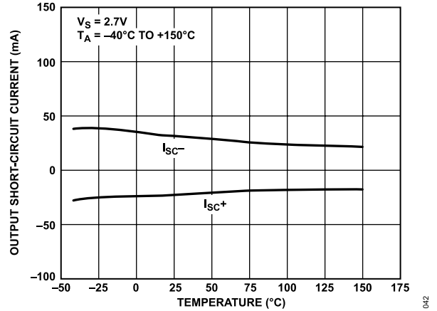
Figure 44. Output Short-Circuit Current vs. Temperature
