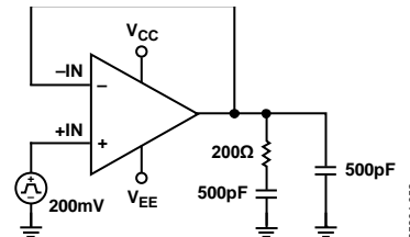
Figure 55. Snubber Network
