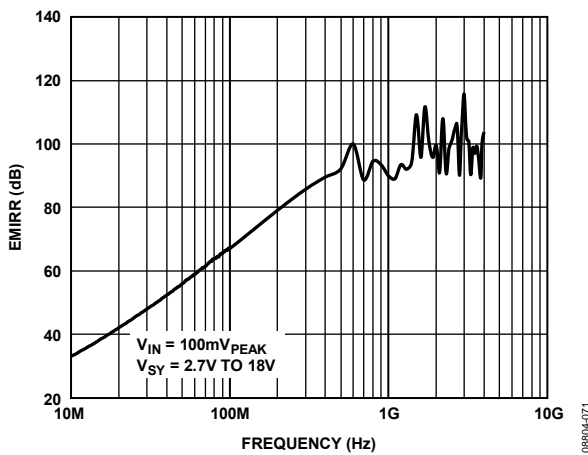
Figure 77. EMIRR vs. Frequency
