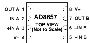
Figure 1. AD8657 Pin Configuration, 8-Lead MSOP
