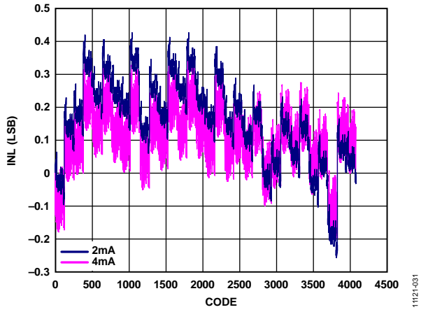
Figure 30. INL, at Two I_{OUTES} Values
