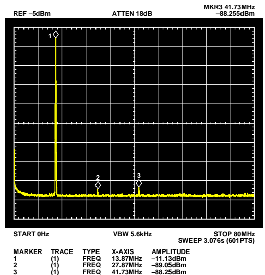
Figure 23. Output Spectrum, f_{OUT} = 13.87 \text{ MHz}
