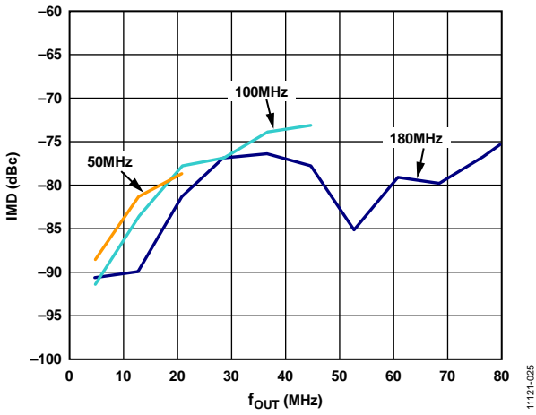
Figure 24. IMD vs. f_{OUT} , at Three f_{DAC} Values
