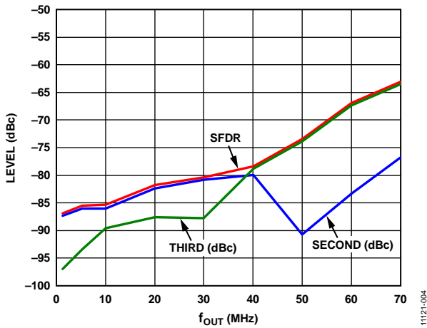
Figure 4. SFDR, Second and Third Harmonics vs. f_{OUT} , I_{OUTFS} = 4\text{ mA}
