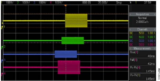
Figure 57. Programming Example 3
