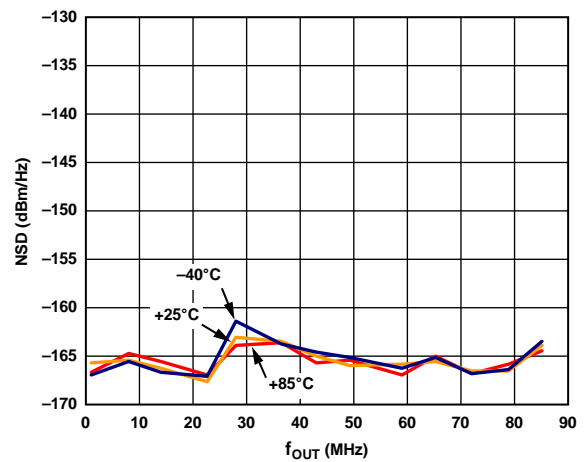
Figure 14. NSD vs. f_{OUT} , at Three Temperatures
