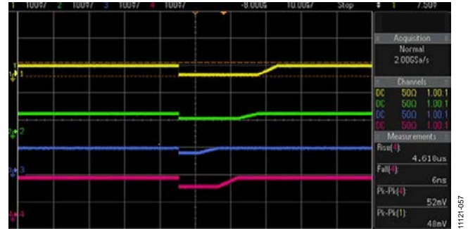
Figure 56. Programming Example 2
