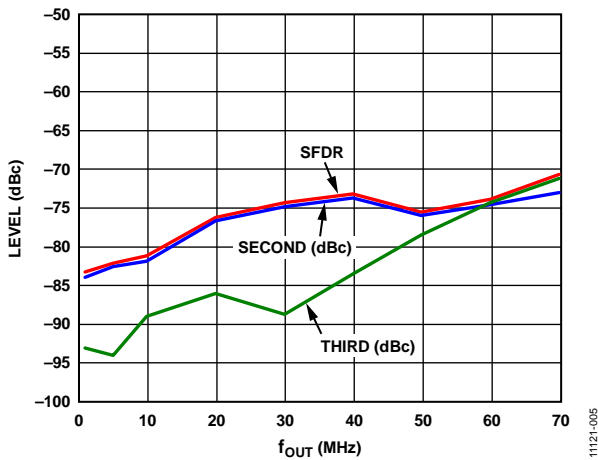
Figure 5. SFDR, Second and Third Harmonics vs. f_{OUT} , I_{OUTFS} = 2\text{ mA}
