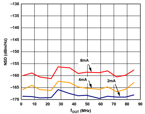
Figure 13. NSD vs. f_{OUT} , at Three I_{OUTFS} Values
