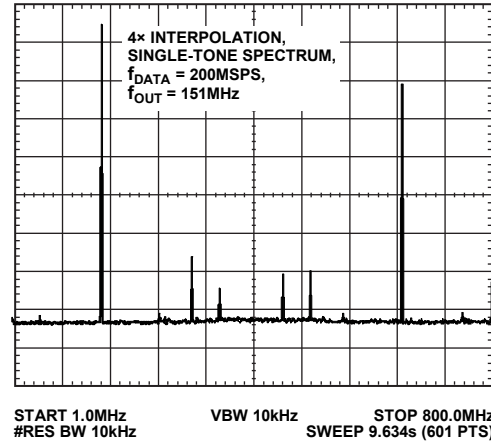
Figure 14. Single-Tone Spectrum, 4x Interpolation, f_{DATA} = 200\text{ MSPS} , f_{OUT} = 151\text{ MHz}
