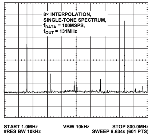
Figure 15. Single-Tone Spectrum, 8x Interpolation, f_{DATA} = 100\text{ MSPS} , f_{OUT} = 131\text{ MHz}
