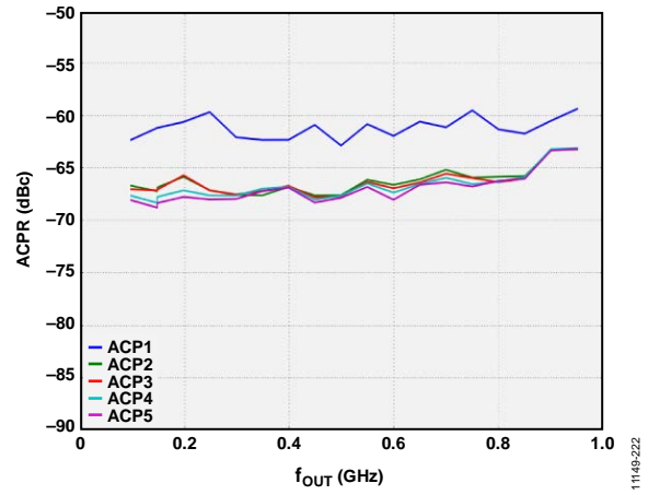
Figure 117. 16-Carrier ACPR vs. f_{OUT}
