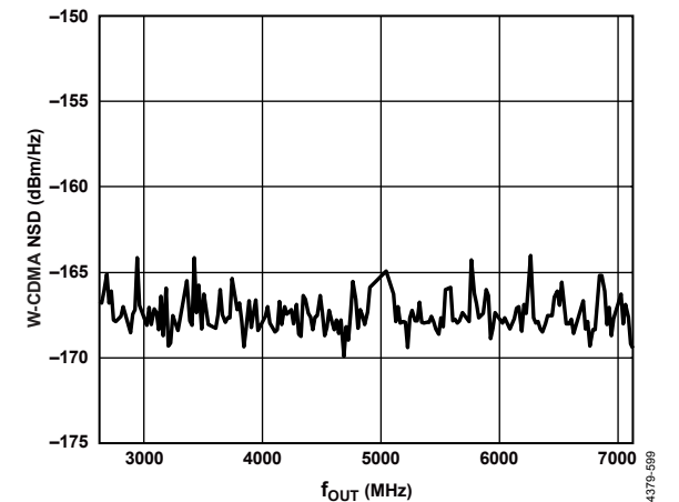
Figure 99. W-CDMA NSD vs. f_{OUT}
