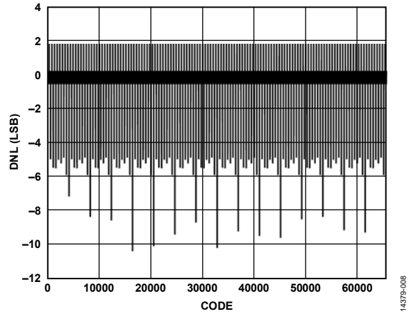
Figure 61. DNL, I_{OUTFS} = 20 mA
